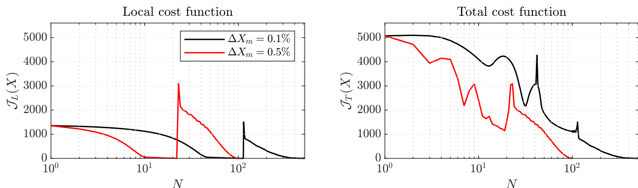
FIG. 8: Cost functions as a function of iteration, N , for small steps ( \Delta X_m = 0.1\% ) and large steps ( \Delta X_m = 0.5\% ).
