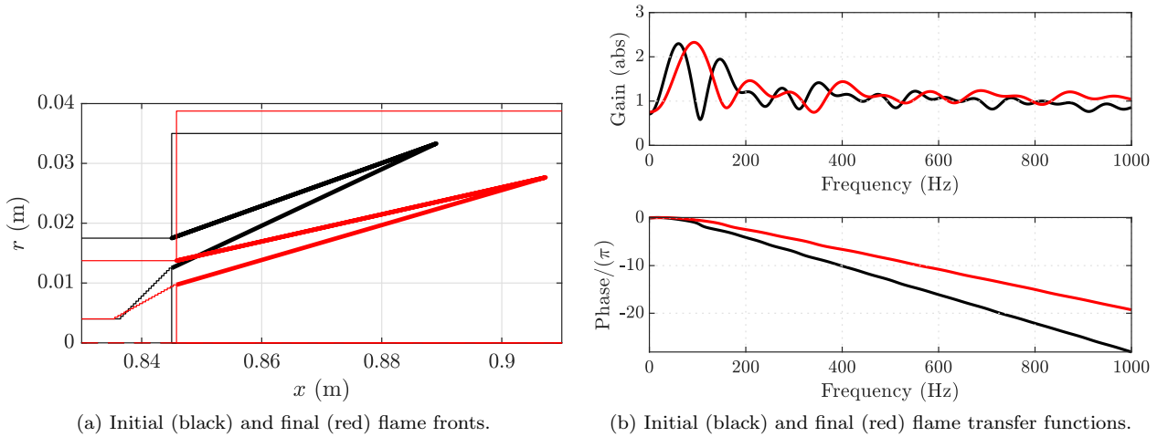
FIG. 11: Diagrams of the initial (black) and final (red) flame fronts and the initial (black) and final (red) flame transfer functions for the optimization process with \Delta X_m = 0.1\% .
