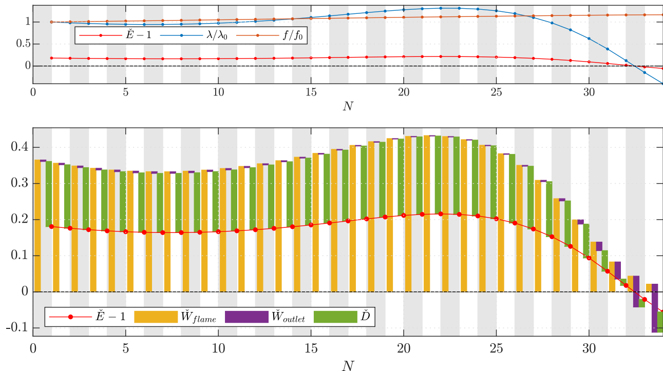
FIG. 13: As in Fig. 12 but for the mode starting at 566 Hz.
