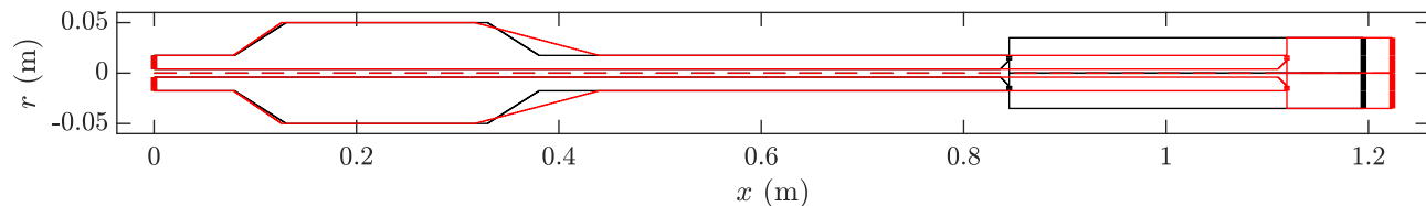
FIG. 14: Plot of the unstable initial (black) and stable final (red) configurations for the optimization routine where only the lengths are allowed to change, except for L_6 .
