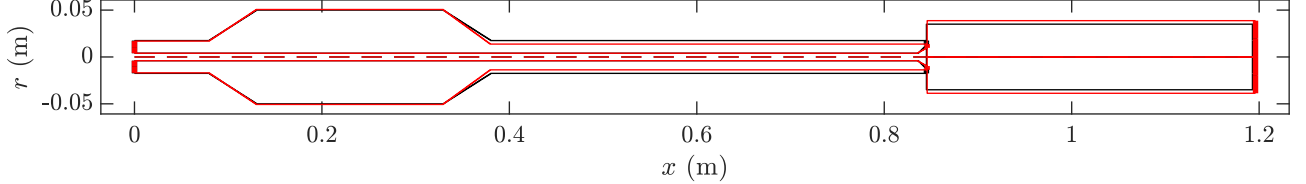
FIG. 10: Plot of the unstable initial (black) and stable final (red) configurations of the longitudinal combustor for the optimization process with \Delta X_m = 0.1\% .
