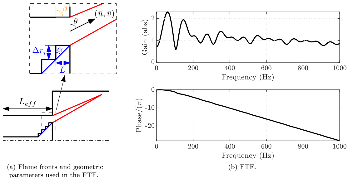
FIG. 2: (a) Geometry of the flame model. The flame fronts are drawn in red, the conical bluff body in blue, and the network model in black. In the network model, the bluff body is modelled as a series of ducts with decreasing area. The angle of the flow between the flame sheets is determined by the last two ducts. (b) The flame transfer function (FTF), which is derived from this flame geometry (see appendix A).
