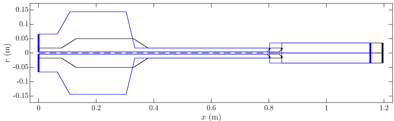
FIG. 16: Original unstable configuration (black) and unstable configuration (blue) obtained using the conjugate gradient algorithm, but without changing any of the parameters controlling the bluff body or combustion chamber.
