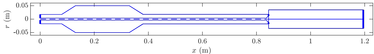
FIG. 17: Original unstable configuration (black) and most unstable configuration (blue) obtained using the conjugate gradient algorithm setting \lambda_o = 200 \text{ s}^{-1} .
