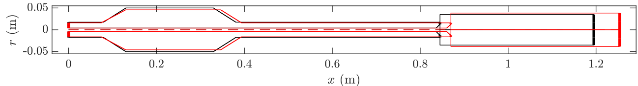
FIG. 15: Original unstable configuration (black) vs stable configuration (red) obtained using a genetic algorithm.
