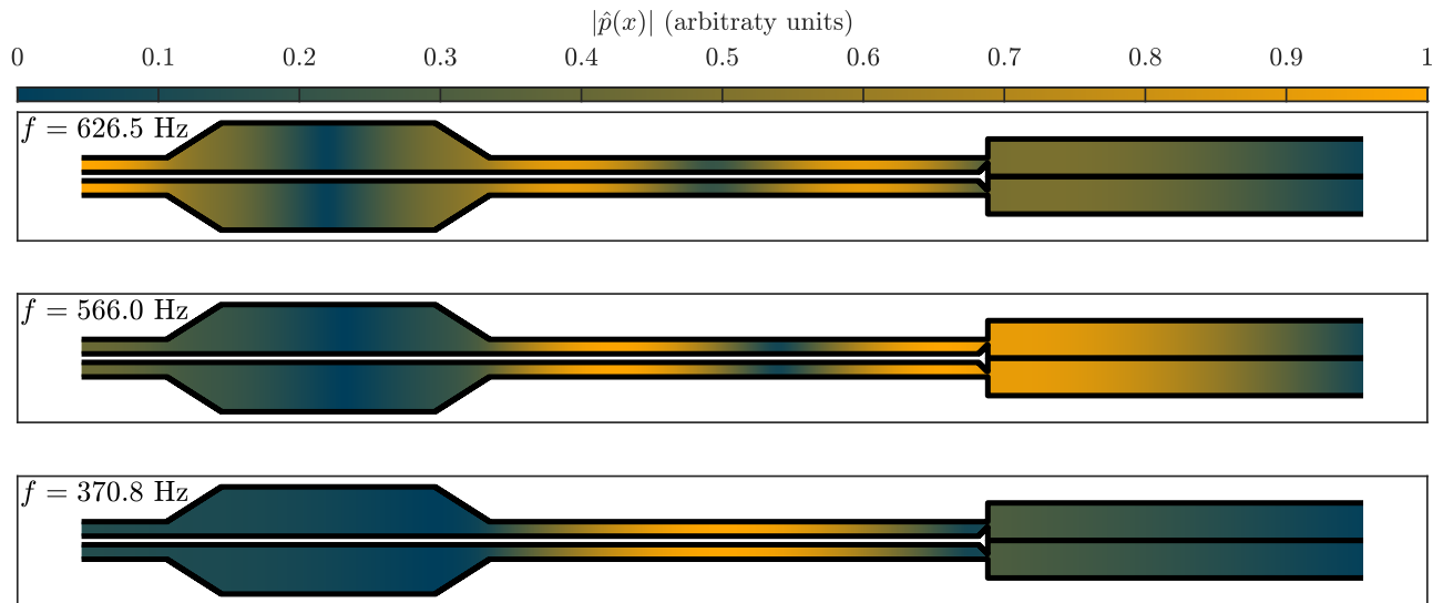
FIG. 4: Modulus of the pressure fluctuations of the 3 most unstable eigenvalues.
