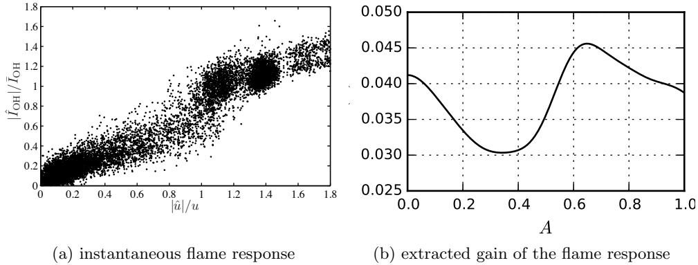
Figure 4: a) instantaneous amplitudes of the dominant Fourier component of OH-chemiluminescence and of the longitudinal velocity at the burner’s position, taken from Moeck et al. (2008). b) Gain modelled. For A \in [0, 1] , the gain was extracted using equation (4.1). The result has then been scaled in both horizontal and vertical axes.
