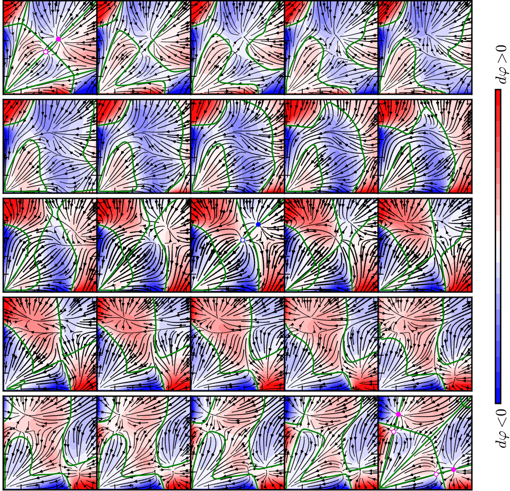
Figure 6: 25 slices of the phase space as presented in Figure 5.b, with the first slice in the top-left corner, ordered to the right and then to the bottom, calculated numerically. This case is for six burners and for \alpha = \alpha_2 = 0.105 as presented in Figure 5.a. In each slice the figure axes are A_1 and A_2 from 0 to \sqrt{2} , with the point (A_1, A_2) = (0, 0) in the bottom-left corner of each slice. The black streamlines represent the two in-plane components dA_1, dA_2 of the vector field, and the color represents the vertical component d\varphi (rescaled). The green lines are contours of d\varphi = 0 . Filled/empty circles are stable/unstable solutions. The top-left and the bottom-right square are at \varphi = 0 and \varphi = \pi , and present standing solutions. The slice in the middle is at \varphi = \pi/2 and presents spinning solutions on the diagonal A_1 = A_2 . The vector field was calculated directly from equations (3.5).
