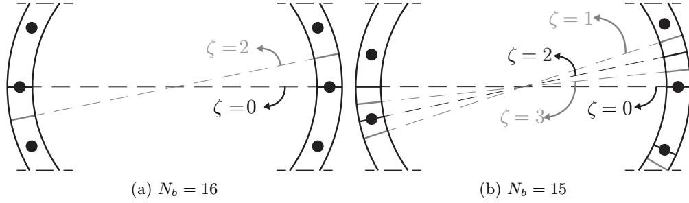
Figure 3: Position of the velocity nodal lines of all possible standing waves in a section of an annular combustor with equispaced burners. We study each of these solutions by fixing the value of \zeta as reported here and in equation (2.2). Each velocity nodal line links two pressure antinodes, and only the lines fully contained in this view are reported. The burners are represented with large black discs, and the semicircles are the internal and external walls of the chamber. In a) the number of burners N_b is even and each burner faces another burner on the other side of the annulus. In the angle \Delta\theta = 2\pi/N_b we have one black and one gray line for a total of 2 standing waves for each burner. In b) the number of burners is odd, and each burner faces the space between two other burners on the other side of the annulus. There are a total of 4 standing waves for each burner. Nonetheless, we can count them only in [0, \pi) , as the modes repeat themselves after a rotation of \pi .
