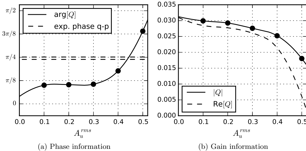
Figure 8: Best reconstruction of the describing function Q of one burner at \omega_s as a function of the pressure oscillation in the annulus, scaled however on the horizontal axis with the local amplitude of the acoustic velocity, for ease of comparison. Available data is dotted, while the lines are obtained with inter-extrapolation. (a) the phase \arg[Q] at a value A_u \approx 0.45 is close to the two values of phase difference between heat release rate and pressure measured experimentally at two azimuthal locations in the annulus. (b) the part of the heat release rate \text{Re}[Q] contributing to the Rayleigh criterion differs significantly from the gain |Q| at large amplitudes. This is because the phase in (a) departs from close to zero as the amplitude increases.
