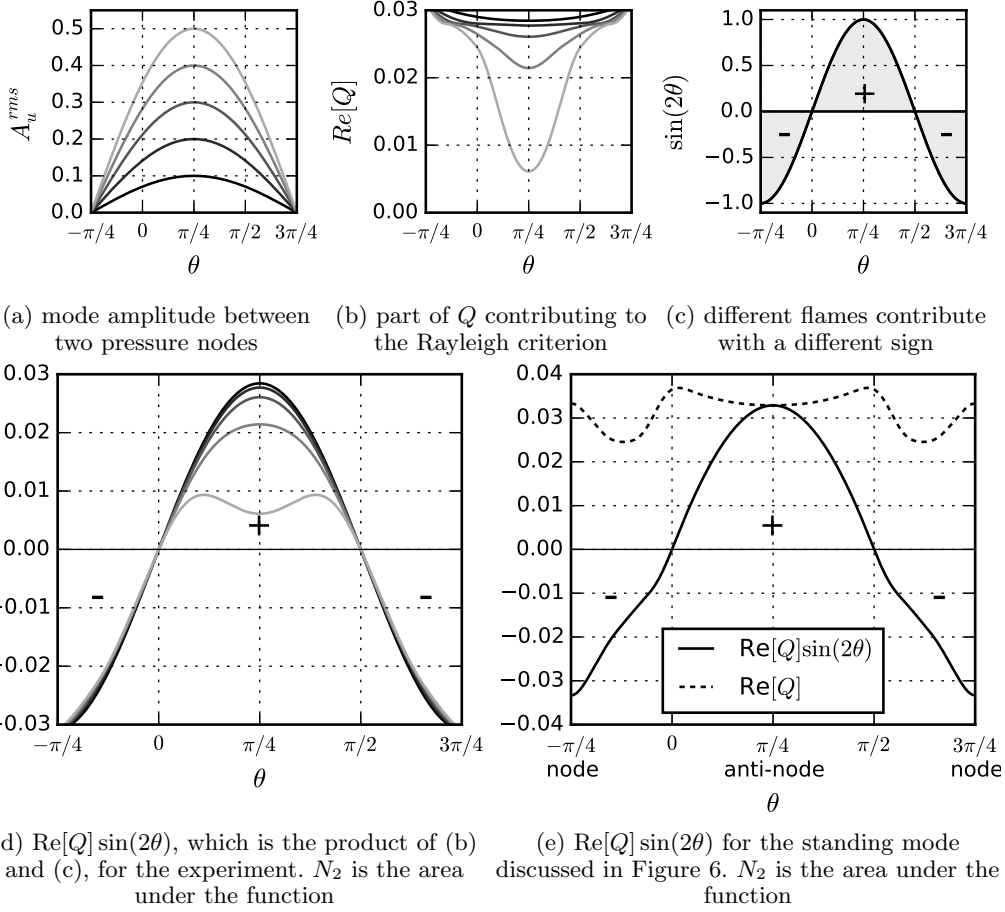
Figure 9: (a) view of the amplitude of the standing mode on one half of the annular chamber, between two pressure nodes at -\pi/4 and 3\pi/4 , with a pressure antinode in the middle. In (a), (b) and (d) we colour results for modes at a larger amplitude with a lighter tone of grey. In (b) we show how on a given line the flames at the pressure antinode respond with a smaller \text{Re}[Q] , consistently with Figure 8.b. This term \text{Re}[Q] is the first factor in the definition (3.24) of N_2 that determines the stability of standing modes. The second factor \sin(2\theta) is reported in (c) and is negative/positive at pressure nodes/antinodes where flames respond respectively in the linear/nonlinear regime. In (d) we report the integrand that defines N_2 . By eye one observes that the positive part is smaller than the negative part, especially at large amplitudes, so that the overall integral N_2 is always negative, and a standing solution at each of the amplitudes would be unstable. In (e) we present for comparison with (d) the integrand defining N_2 for the standing solution presented in Figure 6, which leads instead to a stable standing solution.
