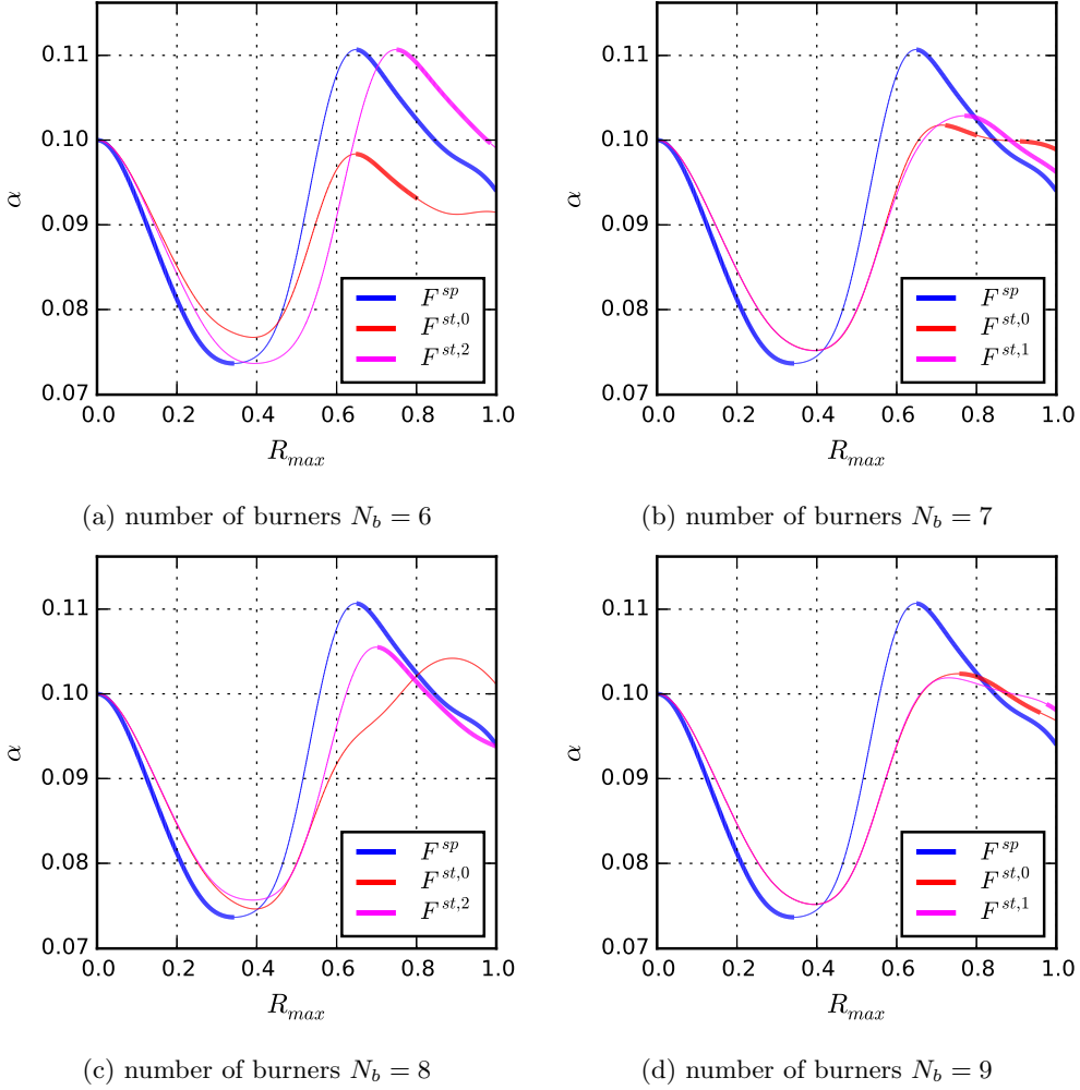
Figure 7: Stability map of a rotationally symmetric annular combustor, for different numbers of burners N_b in each sub-figure. The horizontal axis is the maximum amplitude of azimuthal modes found in the combustor, and the vertical axis is the level of acoustic damping. This analysis is a generalization of Figure 5.a for all values \alpha . The lines are thick/thin if the respective solution is stable/unstable. There exist values of the damping \alpha for which only spinning solutions exist, e.g. \alpha = 0.105 in d).
