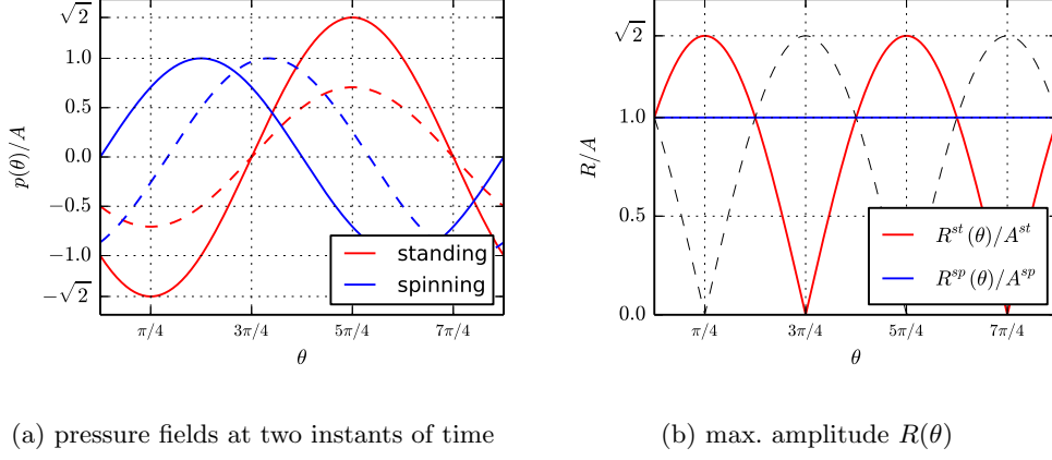
Figure 2: a) Pressure field of a spinning wave (blue) from equation (3.9) and of a standing wave (red) from equation (3.11). b) Amplitude of pressure oscillation of a standing wave (red line) from equation (3.13) and of a spinning wave from equation (3.10). This amplitude of oscillation is responsible for nonlinear saturation effects at the discrete angles \theta_j where the burners are positioned. We also report with a dashed line the amplitude of the acoustic velocity of the standing mode for completeness. For a spinning wave, in a) one observes that in one period of oscillation every point in the annulus experiences the same pressure variation, as the wave rotates and makes a full revolution in one period. This is consistent with R^{sp} in b), where the amplitude of oscillation of a spinning wave is constant. For a standing wave, in a) one observes that different azimuthal positions experience different amplitudes of fluctuating pressure. This can be checked with R^{st} in b), where the amplitude of R^{st} is zero at the position of the pressure nodes in a).
