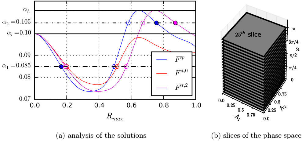
Figure 5: (a) We consider two combustors equipped with six equal burners that differ only in the acoustic damping coefficient \alpha_1 and \alpha_2 , presented with the two dashed and dashed dotted horizontal black lines. We present the amplitude of oscillation R_{max} of spinning (blue) and standing (red/magenta) solutions. The solutions for the two combustors are the intersections, which are presented with filled/empty circles if the solutions are respectively stable/unstable. (b) sketch of the equi-spaced slices of the phase space at constant values of \varphi = k\pi/25 , for k = 0, \dots, 24 presented in Figure 6.
