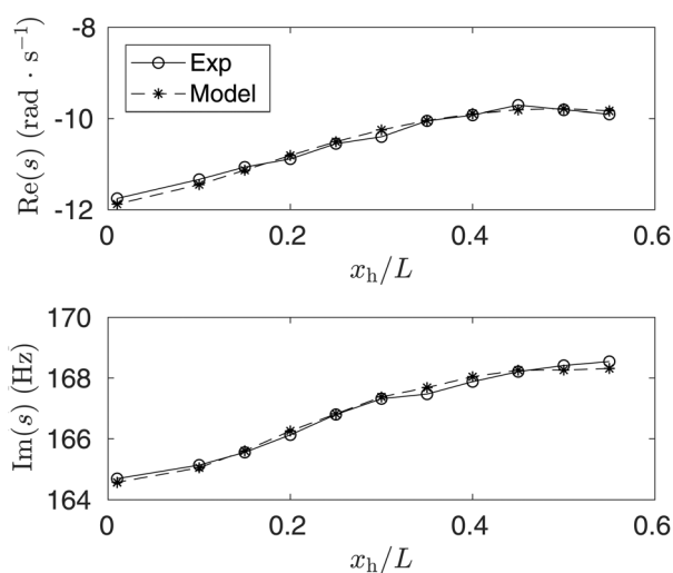
Fig. 8 Decay rate (top) and frequency (bottom) of acoustic oscillations when the heater is switched off and placed at different x_h/L , and thermocouples present inside the tube. The calibrated thermocouple parameters are: k_{vis,t} = 0.257 \text{ kg m}^{-2} \text{ s}^{-1} , k_{th,t} = 1.44 \times 10^{-7} \text{ kg}^{-1} \text{ m}^2 \text{ s} .
