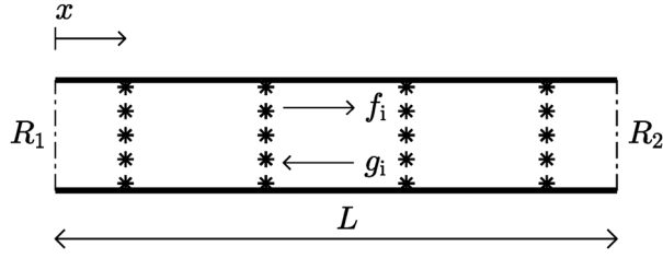
Fig. 6 Sketch of a network model with five acoustic elements separated by four jump conditions. The traveling waves in each acoustic element are denoted by f_i and g_i . R_1 and R_2 are the inlet and outlet reflection coefficients.
