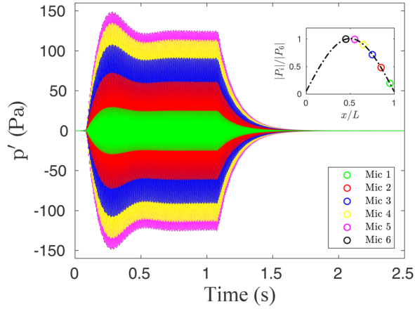
Fig. 3 Pressure oscillations recorded by the six microphones after sinusoidal forcing at 170 Hz. The inset figure shows the corresponding pressure eigenmode.
