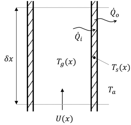
Fig. 4 Sketch of a small element of tube of length \delta x with gas speed U(x) , gas temperature T_g(x) , solid temperature T_s(x) , ambient temperature T_a , and inner and outer heat flow rates \dot{Q}_i and \dot{Q}_o , respectively
