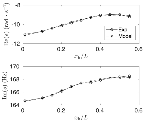
Fig. 7 Decay rate (top) and frequency (bottom) of acoustic oscillations when the heater is switched off and placed at different x_h/L . The calibrated heater parameters are: k_{vis,h} = 27.3 \text{ kg m}^{-2} \text{ s}^{-1} , k_{th,h} = 1.53 \times 10^{-5} \text{ kg}^{-1} \text{ m}^2 \text{ s} , \tau_{vis,h} = -1.36 \times 10^{-3} \text{ s} , and \tau_{th,h} = 8.98 \times 10^{-4} \text{ s} .
