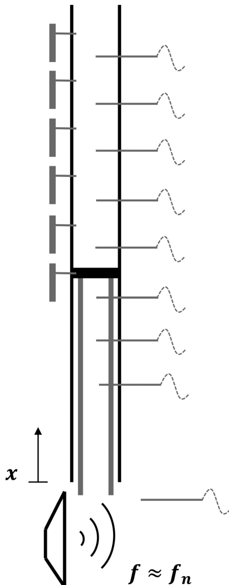
Fig. 1 Sketch of the experimental apparatus including six microphones, eight thermocouples to measure the gas temperature at the tube centerline, a thermocouple to measure the ambient temperature, a loudspeaker, and an electric heater held in place by a pair of prongs and wires. Note that the loudspeaker acoustically forces the system at a frequency, f , close to the natural frequency of the tube, f_n .
