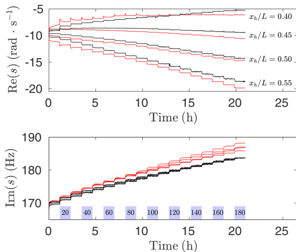
Fig. 10 Decay rate (top) and frequency (bottom) of the oscillations for the case of heater switched on and placed at different x_h/L . The heater power is increased by 10 W every 70 min (bars at the bottom). Red/smooth lines: model. Black/noisy lines: experiments. Optimal thermoacoustic parameters: n = 0.271 , k_\tau = 2.04 .
