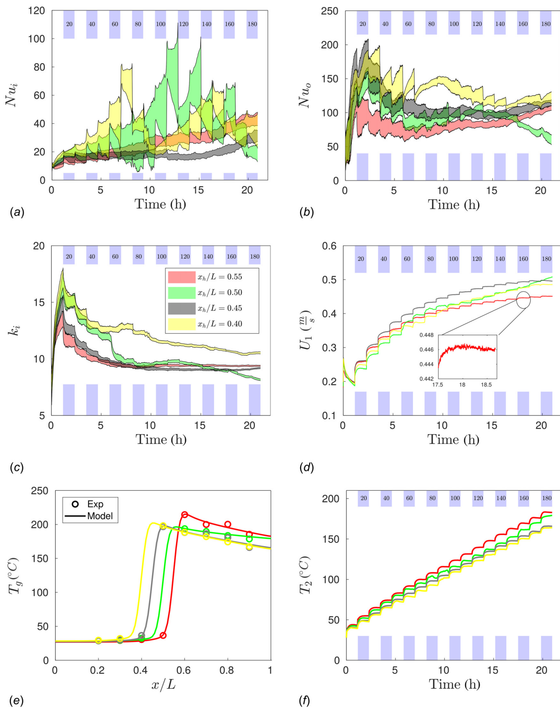
Fig. 5 (a)–(c) Base flow model parameters with uncertainty \pm 2\sigma as functions of time ([h], bottom axis) or heater power ([W], top axis). (d) Bulk velocity of the gas at the inlet of the tube. (e) Gas temperature distribution inside the tube at t = 21 h ( Q_h = 180 W) with corresponding experimental measurements. (f) Outlet gas temperature evolution: (a) inner Nusselt number, (b) outer Nusselt number, (c) pressure loss coefficient, (d) inlet bulk velocity, (e) gas temperature at \tau = 21 h, and (f) outlet gas temperature.
